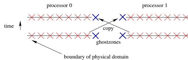
Figure C1.2: Distributed wave equation with ghostzones
